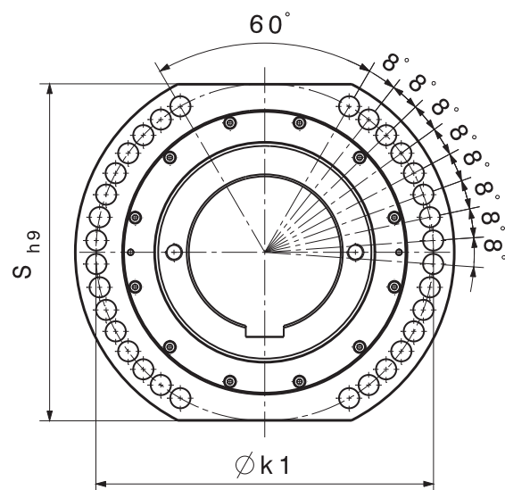
Hole pattern size 800-1030
